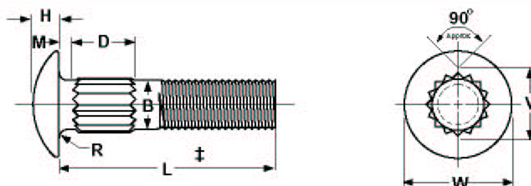
CARRIAGE BOLTS, RIBBED NECK
